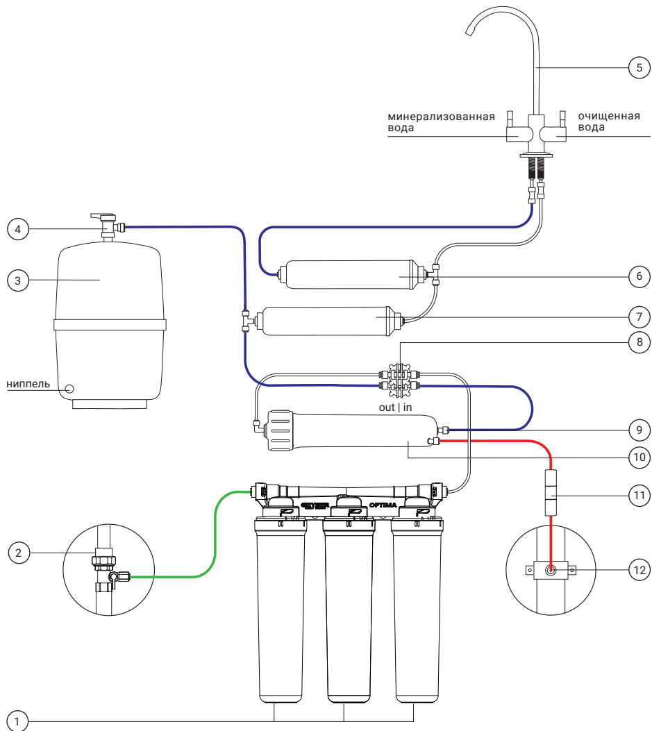
3-rasm. Geyser Zero Optima M ning ulanish sxemasi M [1]
