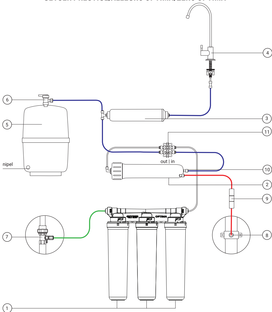
2-rasm. Geyser Prestige/Allegro Optima/Zero Optima uchun ulanish sxemasi
